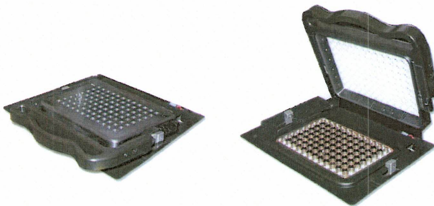
Figure 2 The thermal block assembly, shown with the lid closed (left) and opened (right).
