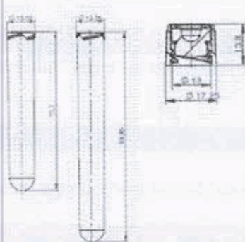
Provetta 13x75 e 13x100, a vite
